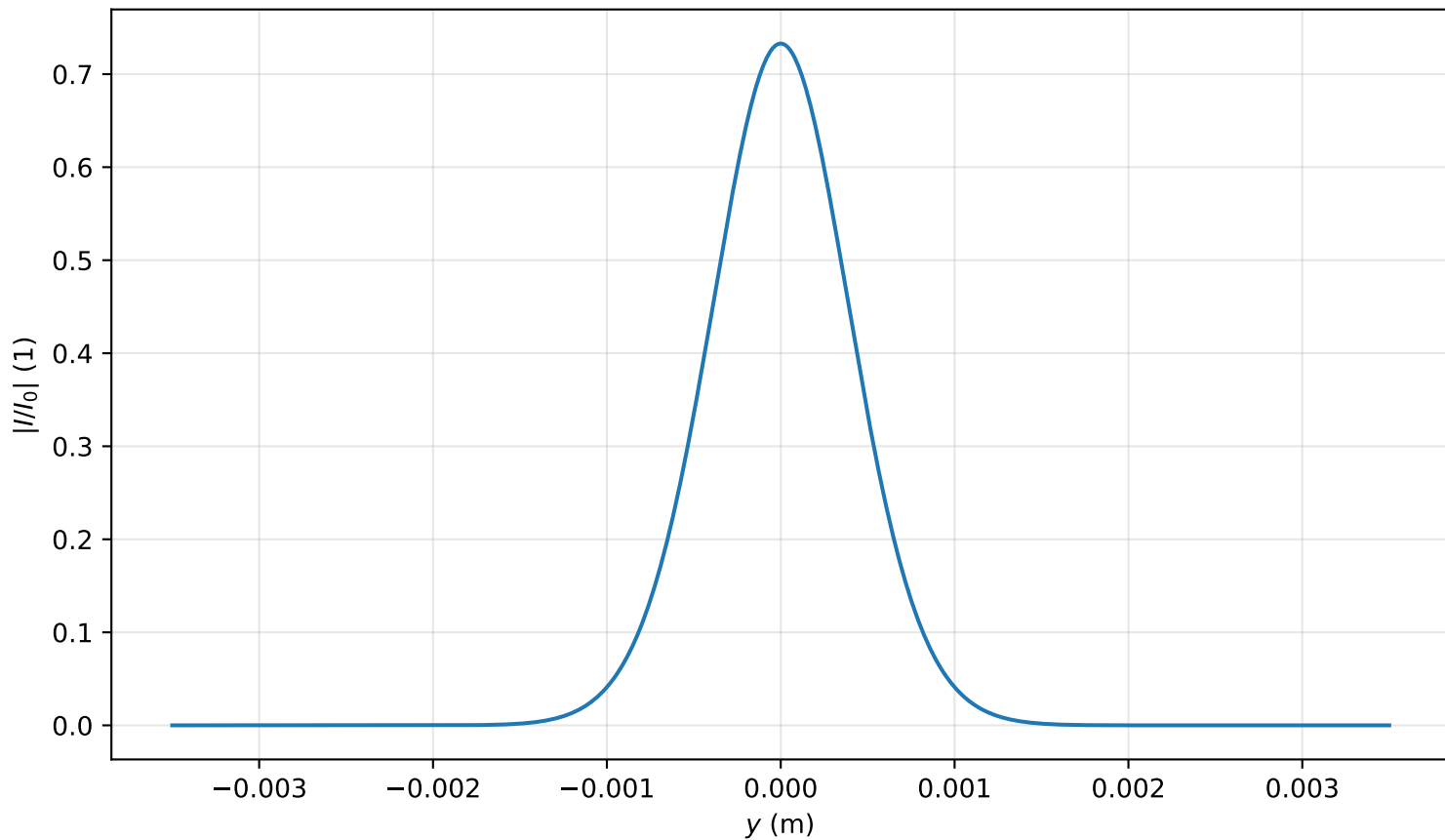
Intensity profile I(x=0, y, z=1.513)/I_0 , \text{Pin}=0.2\text{Pcr} , artificial time
